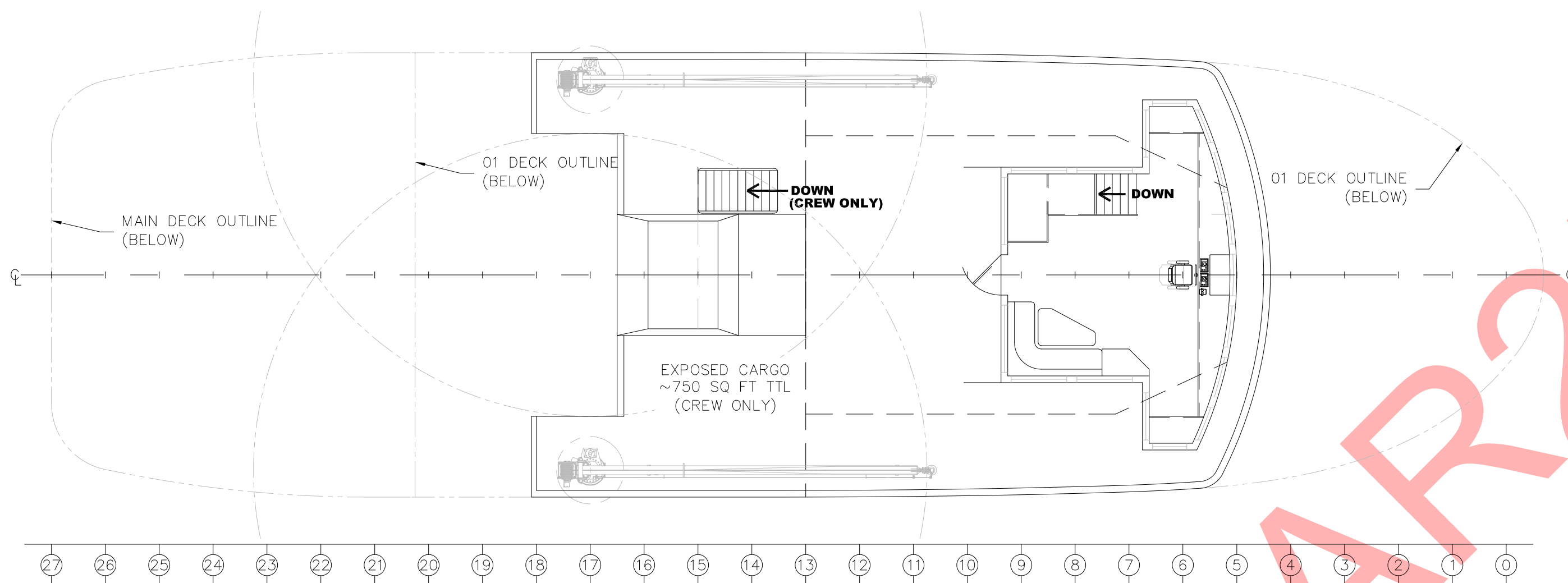
02 DECK PLAN (CREW ONLY)
