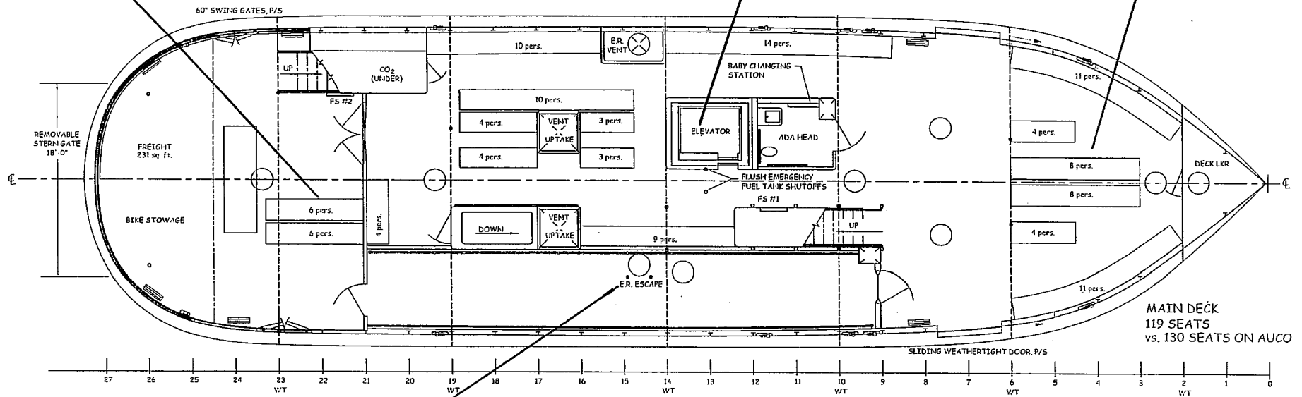
PLAN VIEW, MAIN DECK
